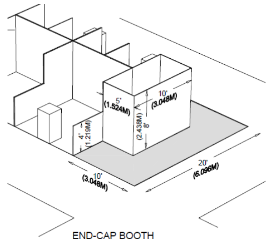
END-CAP BOOTH
